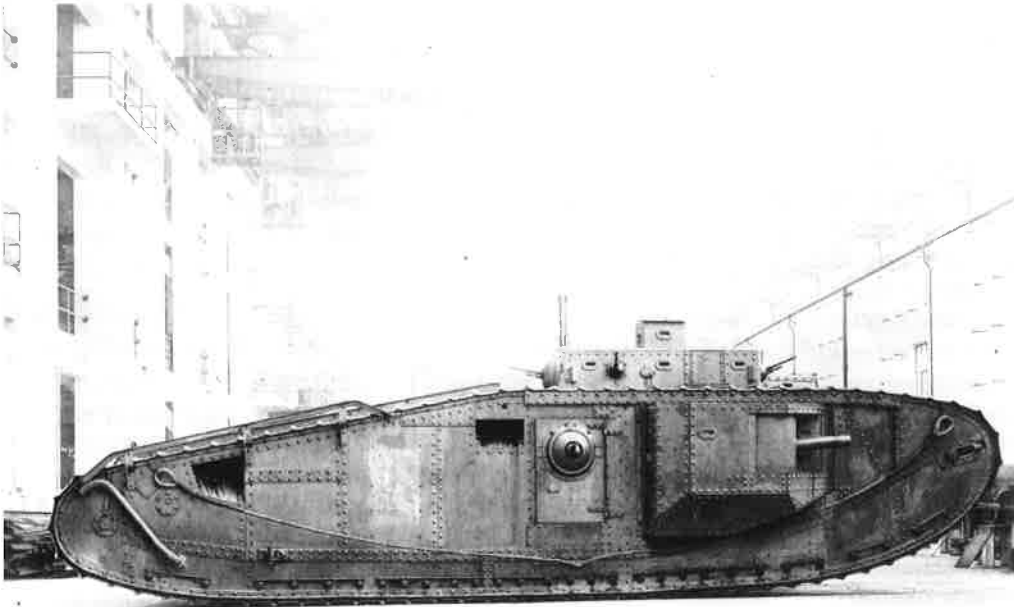
ROCK ISLAND ARSENAL 373-32396 May 22, 1918 Mark VIII Machine; in driveway of Shop "M".
