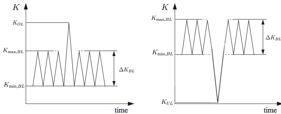
Figure 3. Load parameters for a simple loading scheme, [17].
