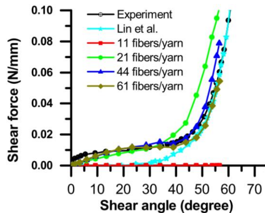
Figure 4: The shear behaviour of Chomarat 150 obtained from the picture frame test and numerical simulations.
